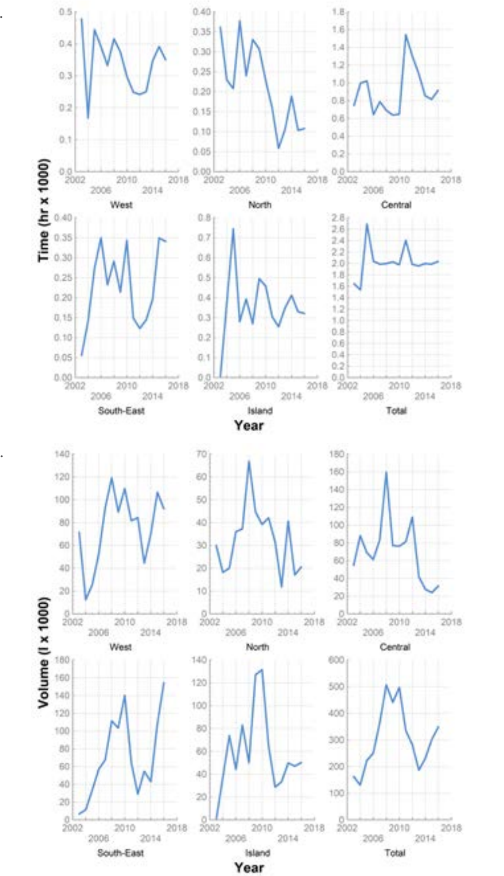
Figure 6.32: Marine litter collected by the Watercare Harbour Clean-up Trust in the Hauraki Gulf / Tīkapa Moana / Te Moana-nui-a-Toi between 2003 and 2016, showing (a) the time worked by the Trust’s staff, and (b) estimated volumes of marine litter collected. Note that the y-axis varies among graphs. Data provided by H. Smith, Sea Cleaners.
