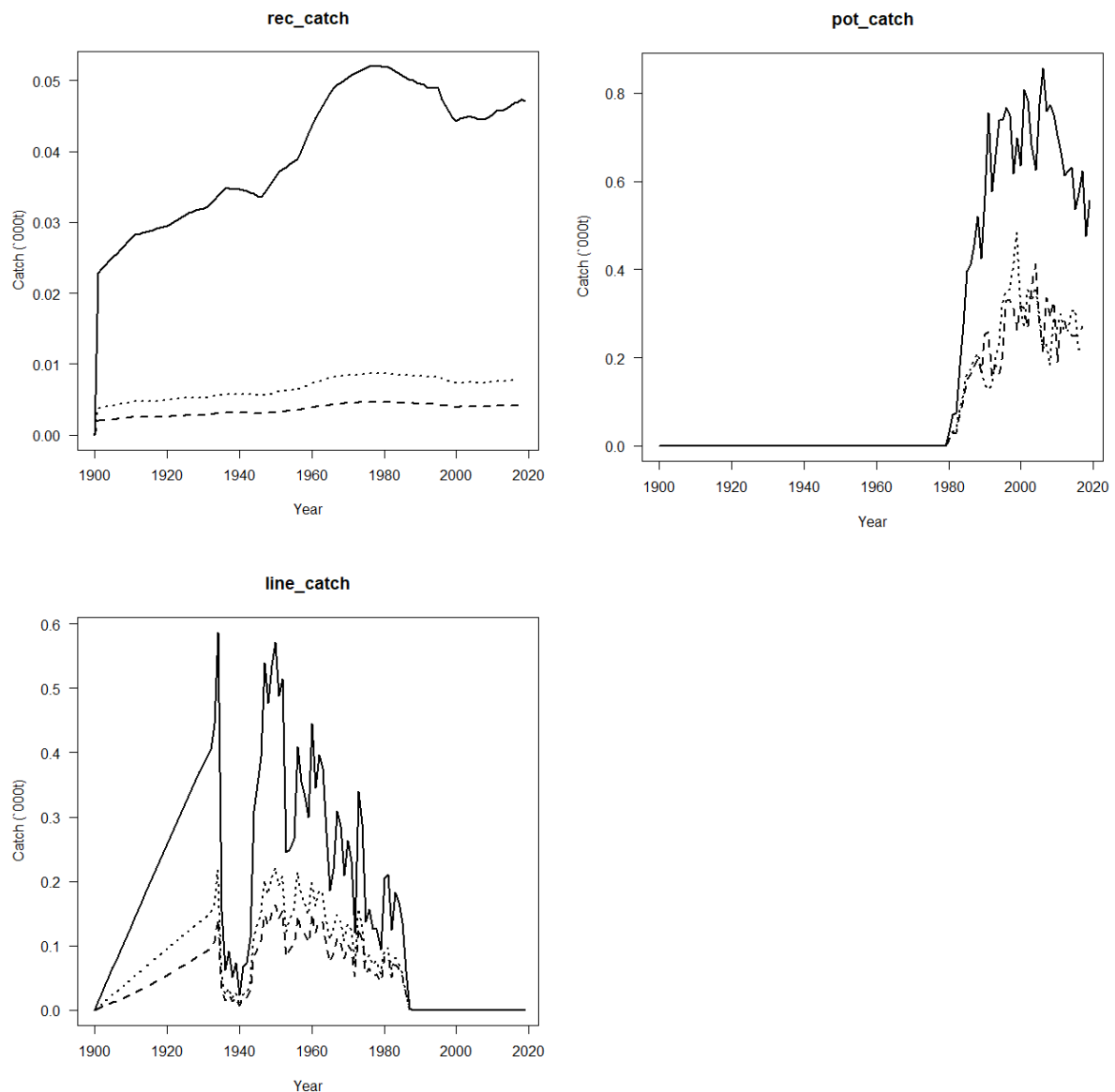
Figure 13: Constructed catch history used in the assessments by fishery and Statistical Areas 025 (solid line), 027 (dashed line), & 030 (dotted line).
