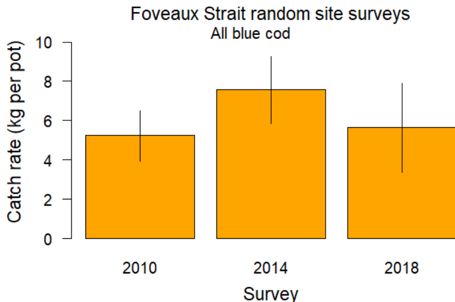
Figure 8: Foveaux Strait random-site potting survey catch rates of all blue cod by survey year. Error bars are 95% confidence intervals.
