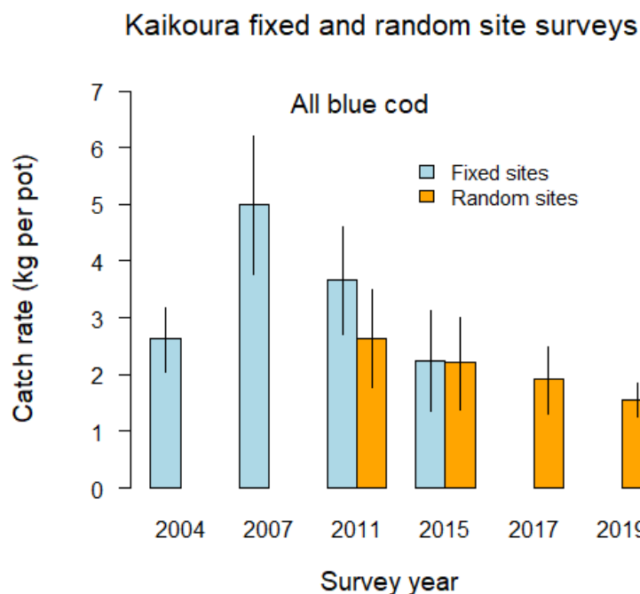
Figure 4: Kaikōura fixed-site and random-site potting survey catch rates of all blue cod by survey year. Error bars are 95% confidence intervals.
