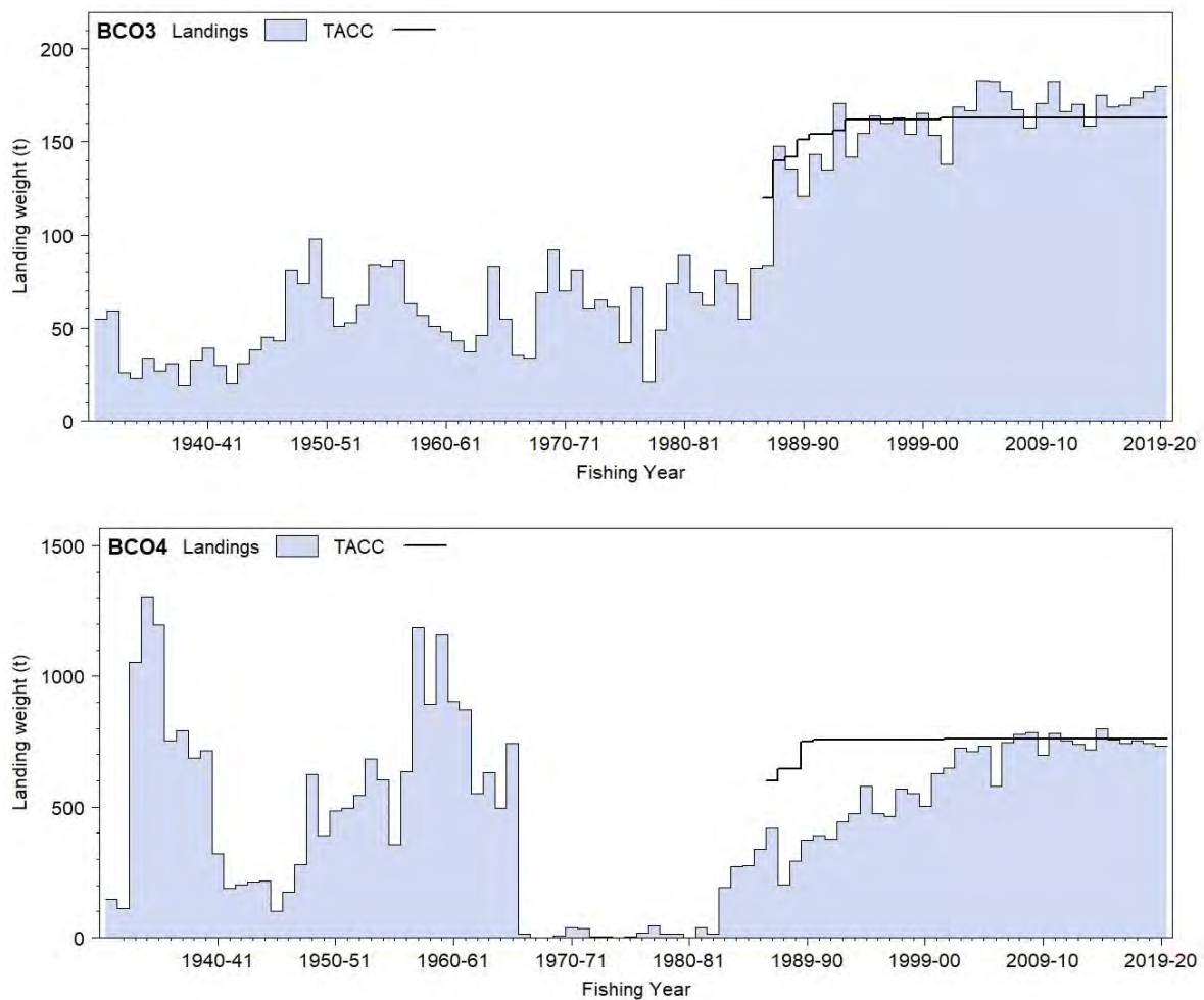
Figure 1: Reported commercial landings and TACC for the five main BCO stocks. From top: BCO 3 (South East Coast) and BCO 4 (South East Chatham Rise). [Continued on next page]
