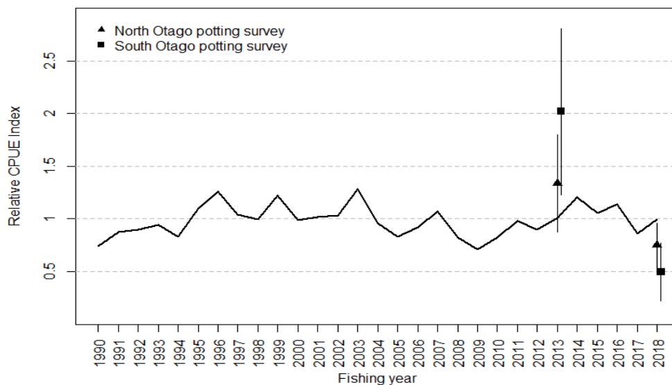
Figure 11: Comparison of BCO 3 standardised series (1989–90 to 2017–18) based on landed green weight catch data and the 2013 and 2018 observations from the North Otago and South Otago potting surveys conducted at random sites over all strata (Large et al in prep a). (Each relative series is scaled so that the geometric mean equals 1.0 from 2013 to 2018.)
