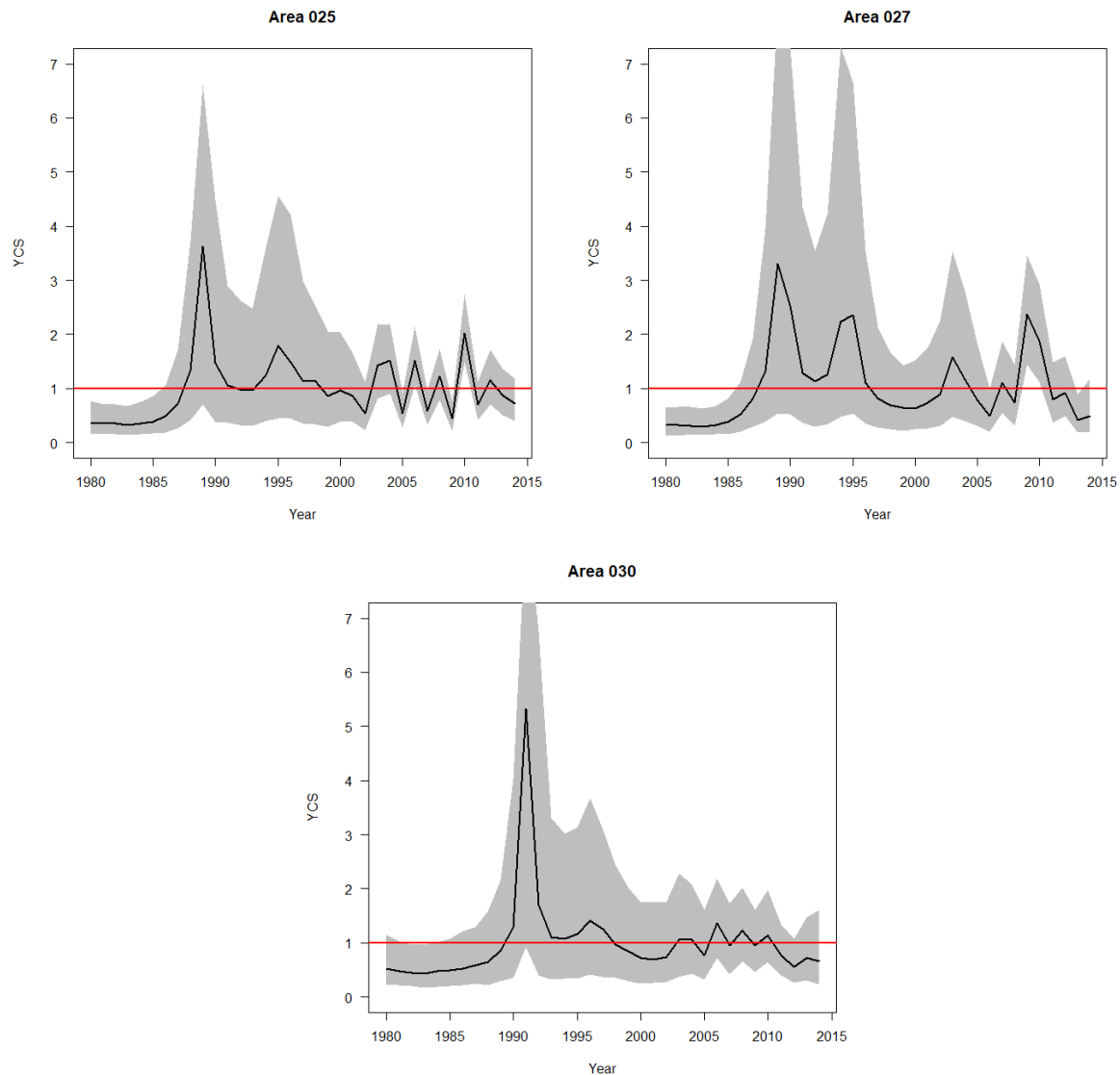
Figure 15: Year Class Strength (YCS) from the base-case runs for Statistical Areas 025, 027, and 030, for 1980–2014. Medians are shown by the black line and the shaded areas show the 95% range limits.
