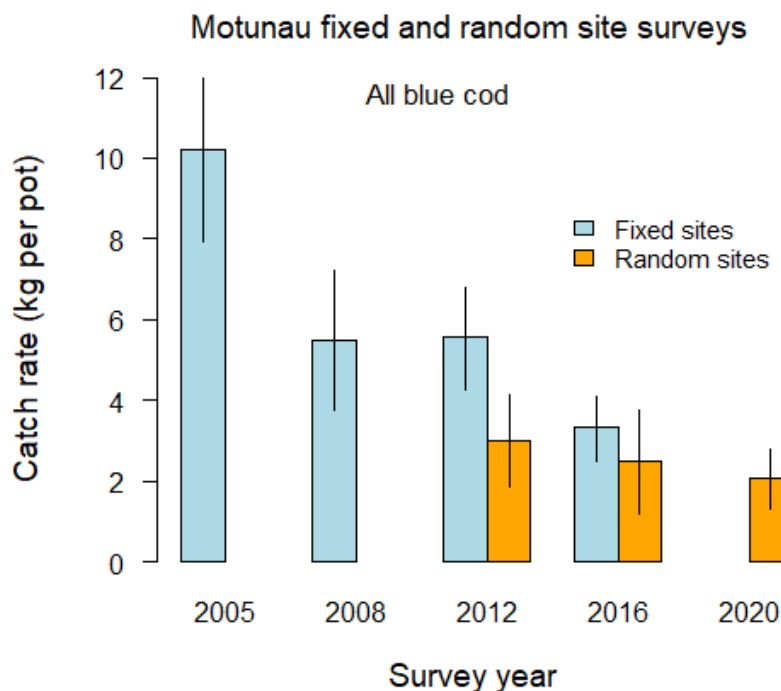
Figure 5: Motunau fixed-site and random-site potting survey catch rates of all blue cod by survey year. Error bars are 95% confidence intervals.
