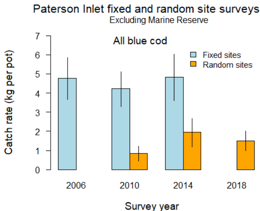
Figure 9: Paterson Inlet random-site potting survey catch rates of all blue cod by survey year. Error bars are 95% confidence intervals.
