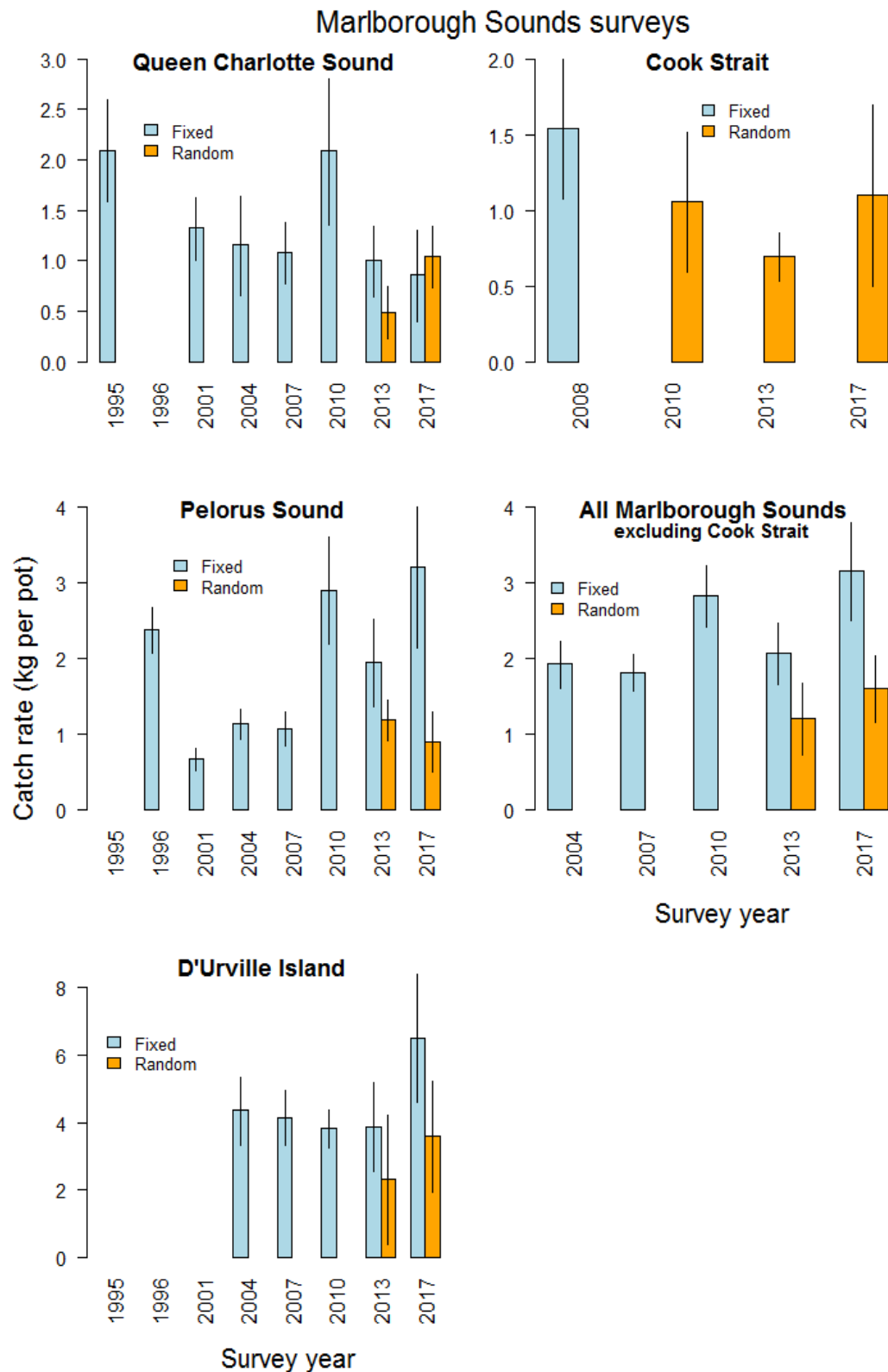
Figure 3: Marlborough Sounds fixed-site and random-site potting survey catch rates of all blue cod by survey year for each region and overall for the Marlborough Sounds. Error bars are 95% confidence intervals. There were no complete fixed-site surveys in Queen Charlotte Sound in 1996, Pelorus Sound in 1996, and D'Urville Island from 1995 to 2001. For the overall Marlborough Sounds plot, the 2004 and 2007 fixed-site surveys exclude Separation Point, and the random-site surveys exclude Cook Strait, hence the strata are consistent among the surveys for fixed and random site surveys.
