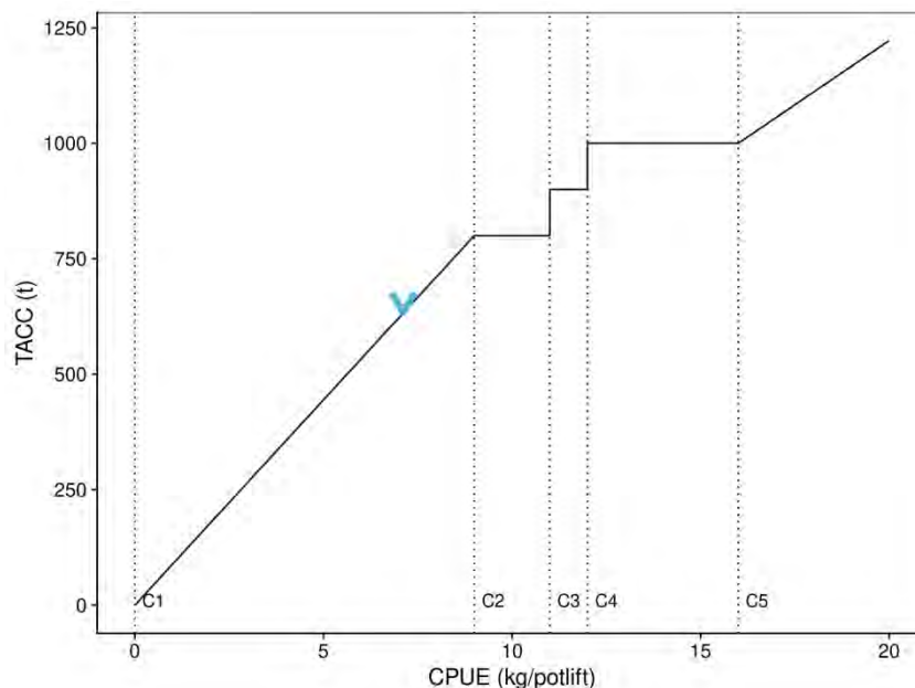
Figure 17: Harvest control rule relating the commercial TACC (t) to catch-per-unit-effort (CPUE, kg per potlift). The control rule is defined by CPUE parameters C1–C5 as well as corresponding TACC levels. The 2020 CPUE level is indicated by the light-blue arrow, suggesting a further reduction in TACC may be necessary to reduce fishing impacts under reduced current productivity.
