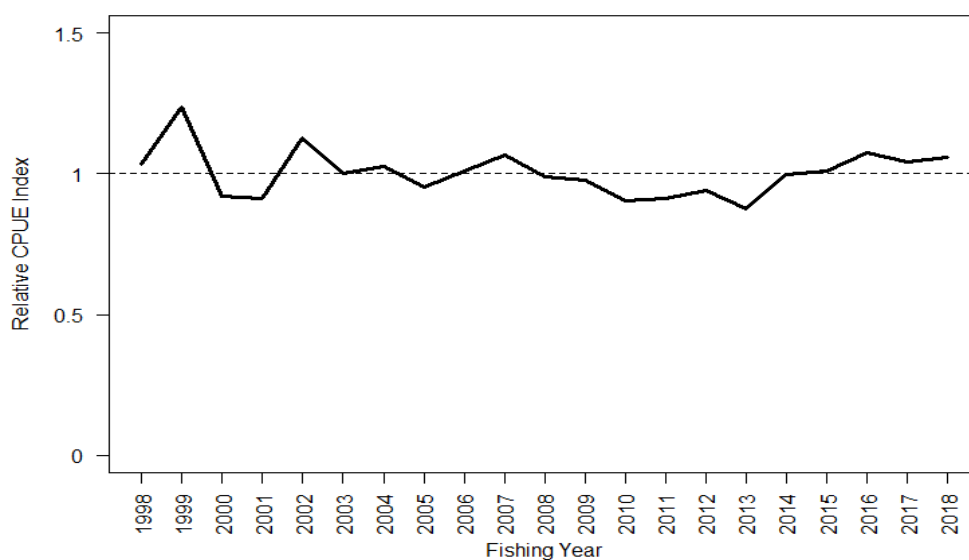
Figure 12: Standardised CPUE index for BCO 4 based on records of positive BCO catch by core vessels, 1997–98 to 2017–18 (Large et al in prep b).
