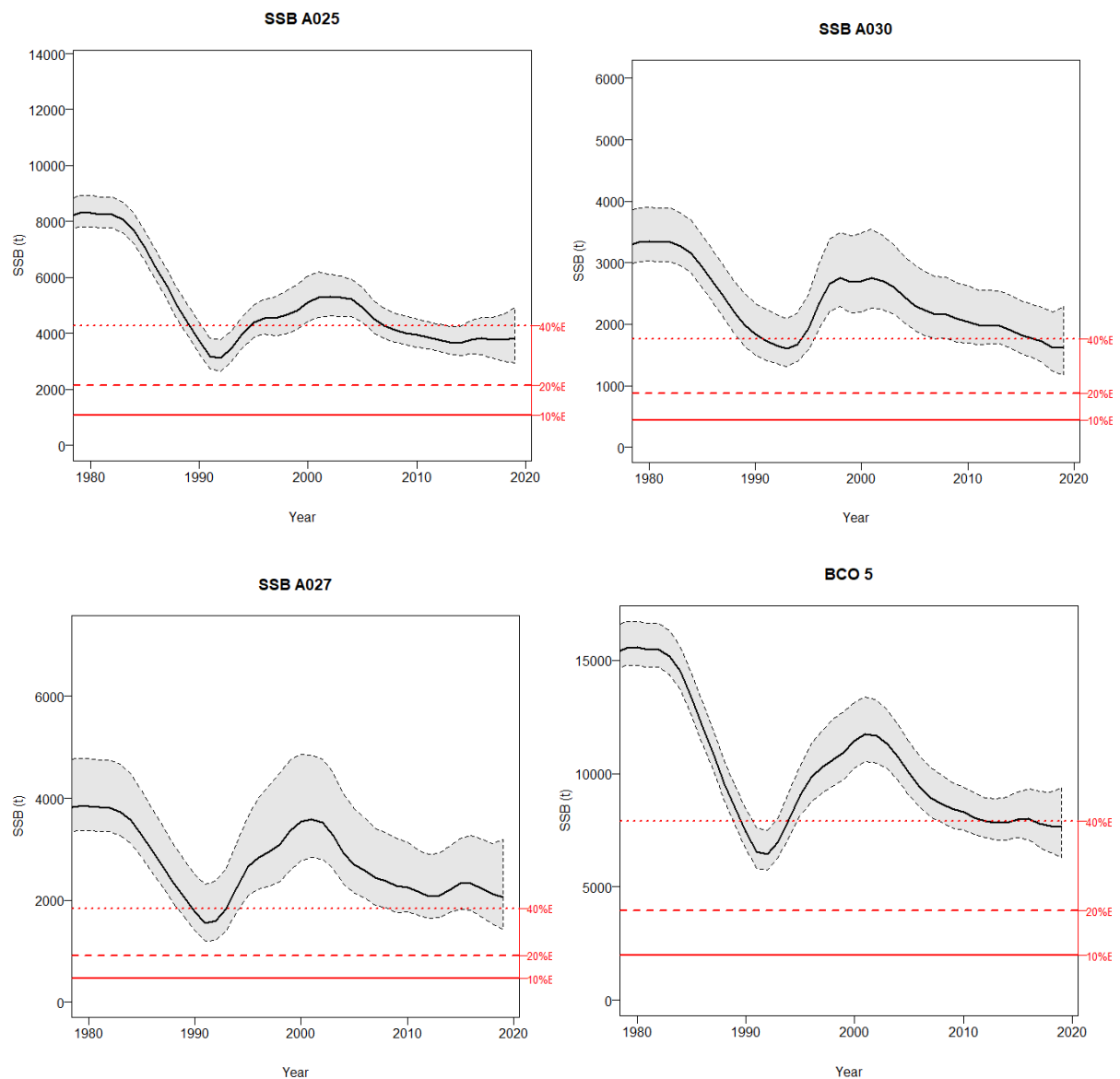
Figure 14: Median estimates of spawning biomass for Statistical Areas 025, 027, and 030, and the three areas combined, for the base-case model runs, 1980–2019.
