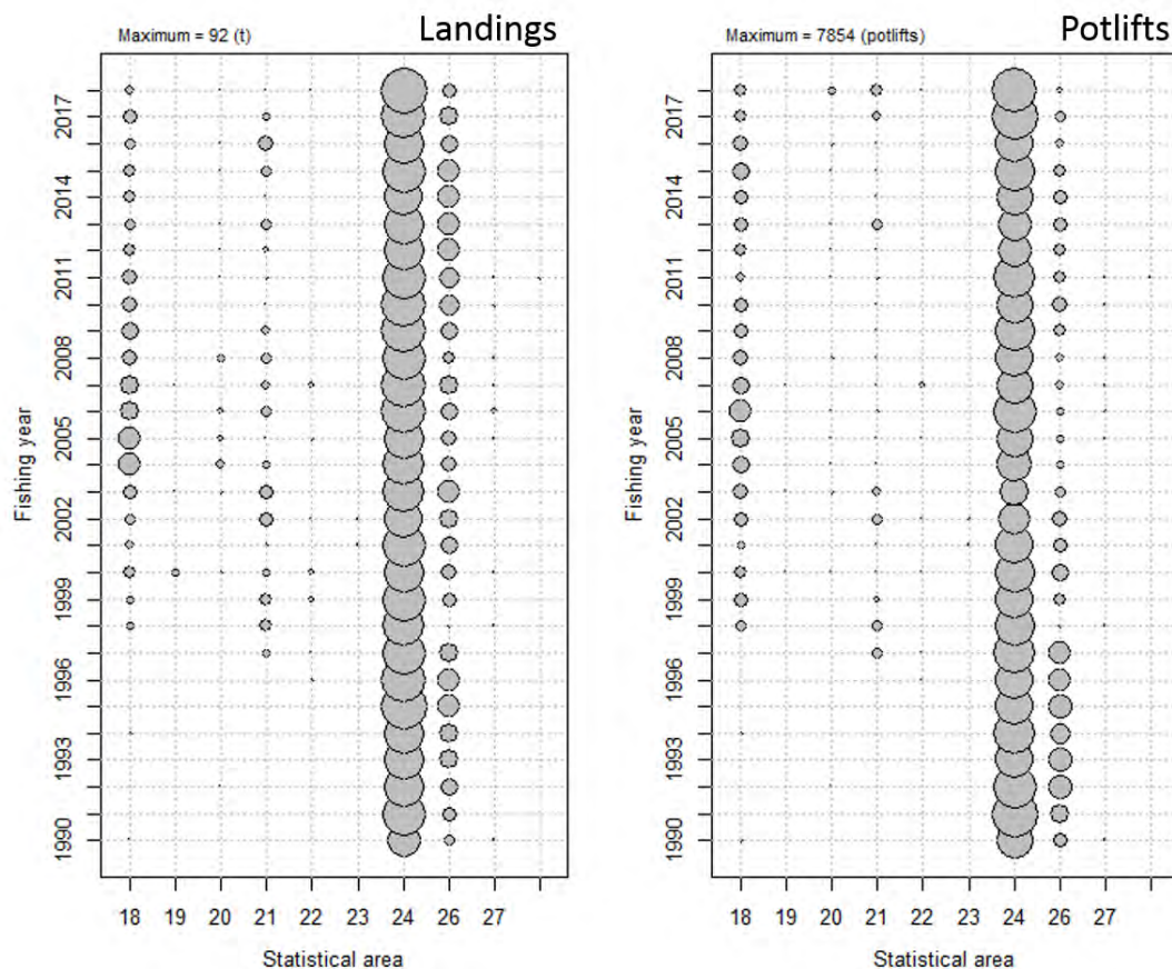
Figure 10: Distribution of landings and number of potlifts for the cod potting method by statistical area and fishing year from trips which landed BCO 3. Circles are proportional within each panel: [landings] largest circle = 92 t in 2011 for 024; [number potlifts] largest circle = 7854 pots in 2006 for 024 (Large et al in prep a).
