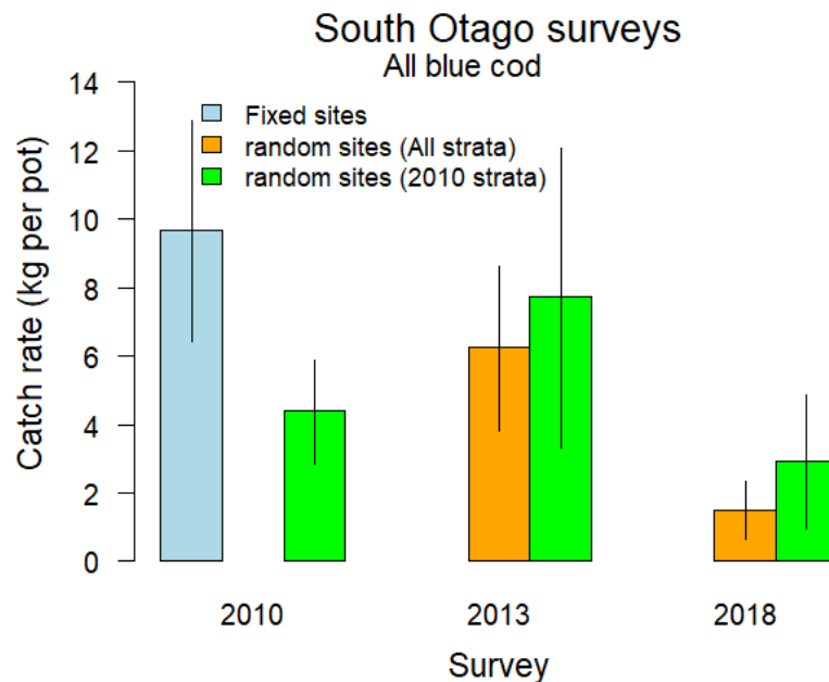
Figure 7: South Otago fixed-site and random-site potting survey catch rates of all blue cod by survey year. Error bars are 95% confidence intervals. The 2010 survey used three strata, and subsequent surveys used 6 strata. Catch rates are also shown for the three strata used in 2010 for the random-site surveys.
