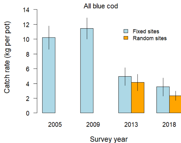
Figure 6: North Otago fixed-site and random-site potting survey catch rates of all blue cod by survey year. Error bars are 95% confidence intervals. Surveys after 2005 include a new stratum (stratum 6).
